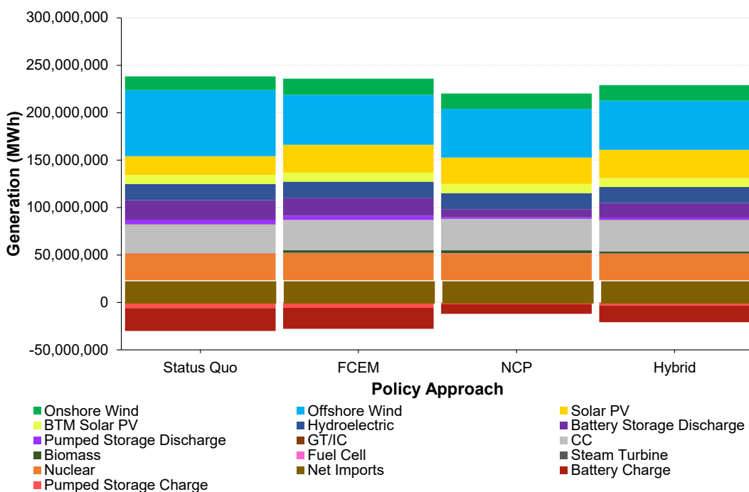
Figure B-A-2. Generation by Technology Type Across Policy Approaches, 2040 (MWh)
