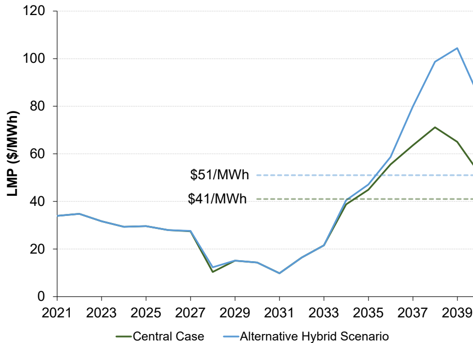
Figure B-B-11. Average Annual LMP, Hybrid Case for Central Case and Alternative LMP Scenario, 2021-2040 ($2020/MWh)
