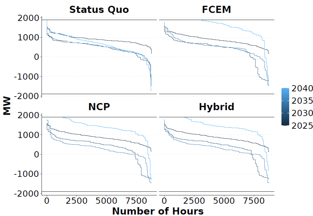
Figure B-B-15. Hourly Power Flows for Maine-New Hampshire, 2025, 2030, 2035, 2040
