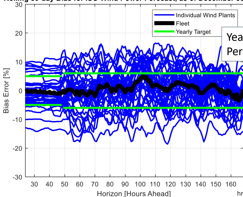
Rolling 30-day Bias for ISO Wind Power Forecast, as of December 30, 2021
