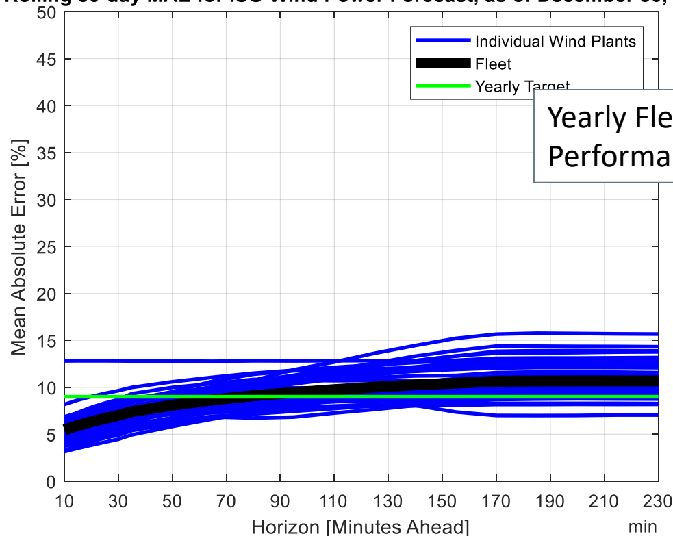
Rolling 30-day MAE for ISO Wind Power Forecast, as of December 30, 2021
