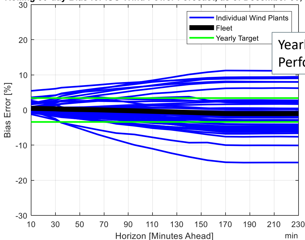
Rolling 30-day Bias for ISO Wind Power Forecast, as of December 30, 2021
